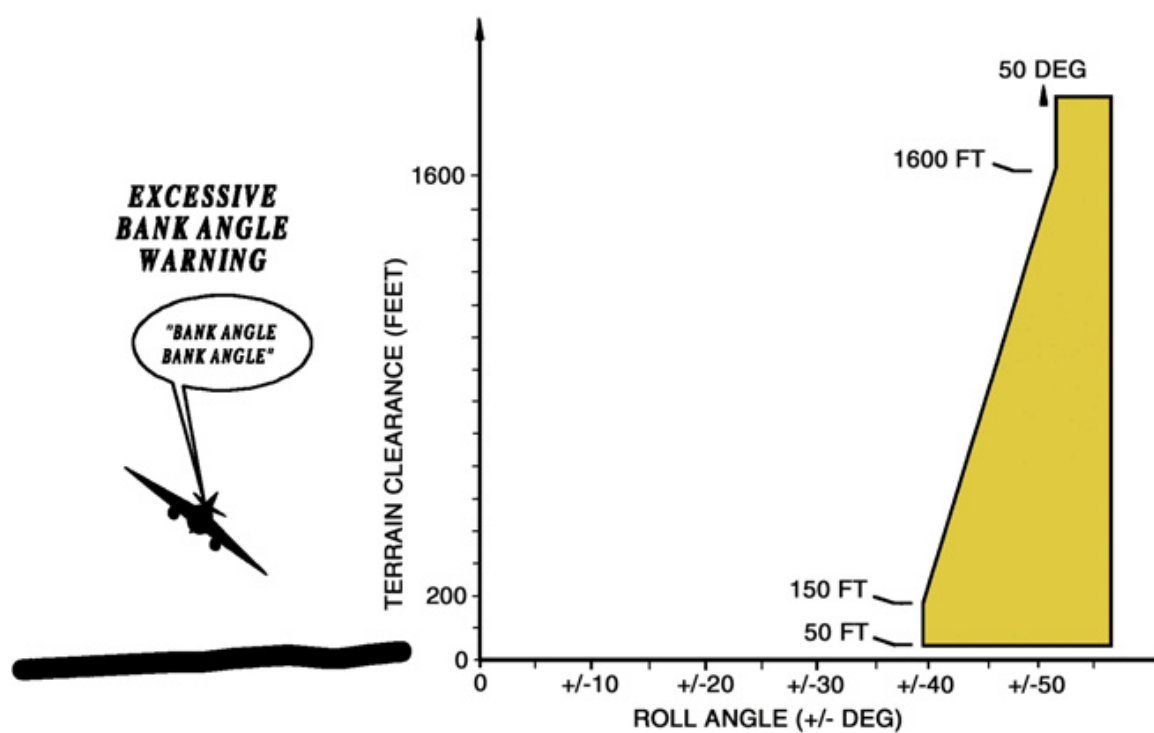
Excessive Bank Angle Alert Envelope
