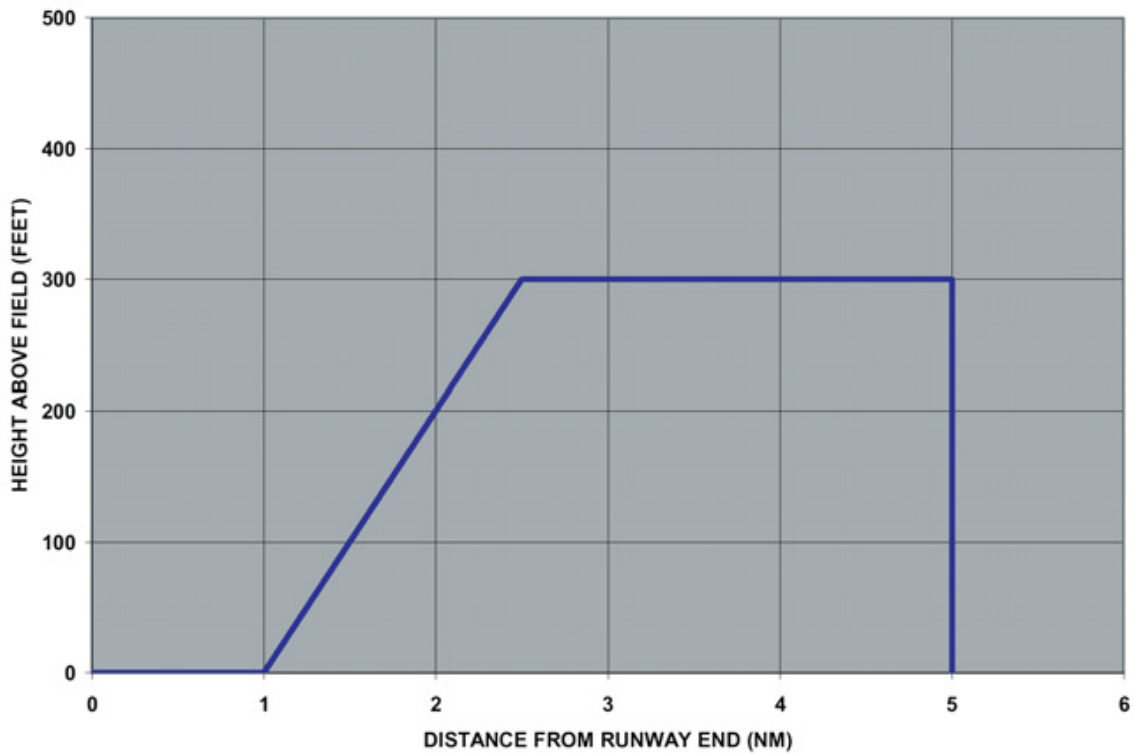
Runway Field Clearance Floor (RFCF)
