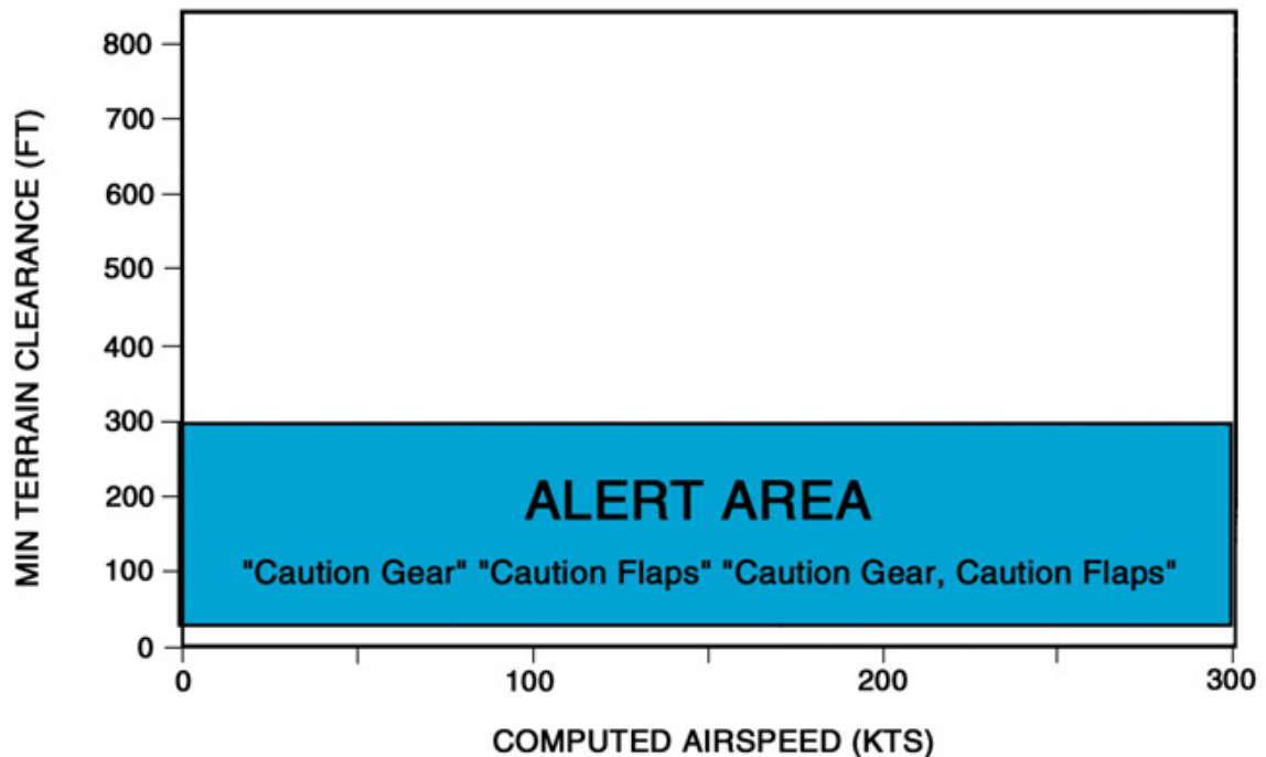
Gear and Flaps Alert Envelope
