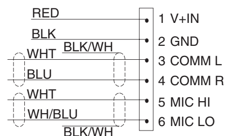
Aircraft Interface Schematic
